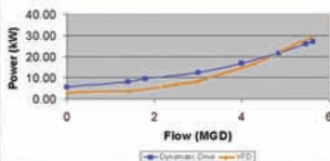
RAS PUMP POWER USAGE COMPARISON TANK 5 40HP Motor 1760RPM - TEST DATE 1/26/2004
