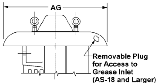
DRIP COVER FOR VERTICAL OPERATION
