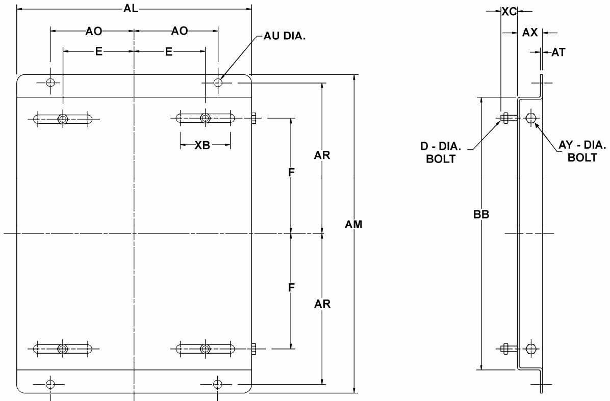
Outline Drawings - Adjustable Slide Bases
