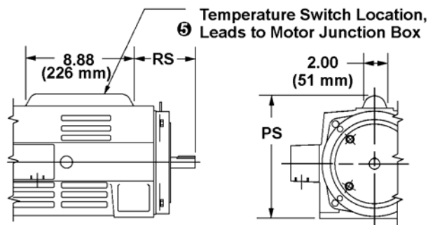
TEMPERATURE SWITCH
