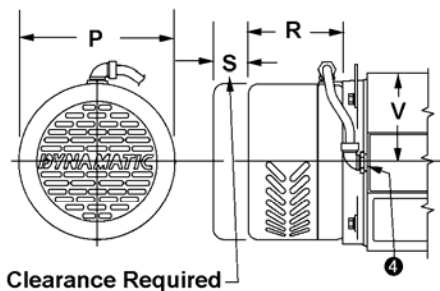
ADJUSTABLE TORQUE BRAKE (EDDY CURRENT BRAKE)
